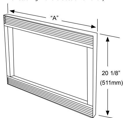
AOCTK OVERALL DIMENSIONS (Epicure™ or Millennia™ Trim Kit - use these models when stacking with the Discovery Wall Oven)
