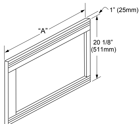
ACTK OVERALL DIMENSIONS (Epicure™ or Millennia™ Trim Kit - use these models when stacking with the Classic Wall Oven)
